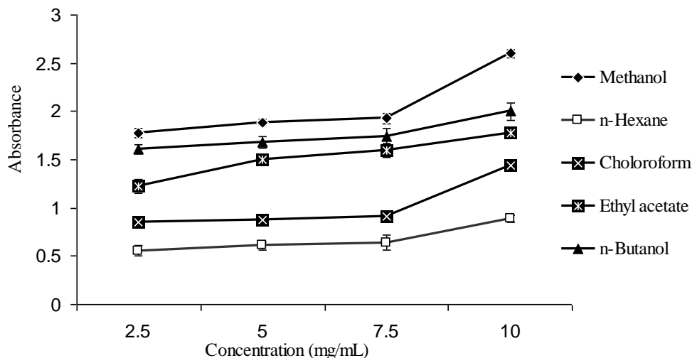
Fig. 1: Reducing potential of Solanum melongena leaves extracts
