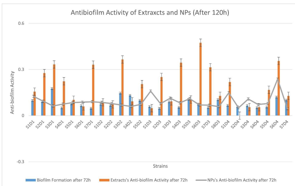
Fig. 2c and 2d: Anti-biofilm activity of plant extract and NPs (After 72 and 120 hours)
